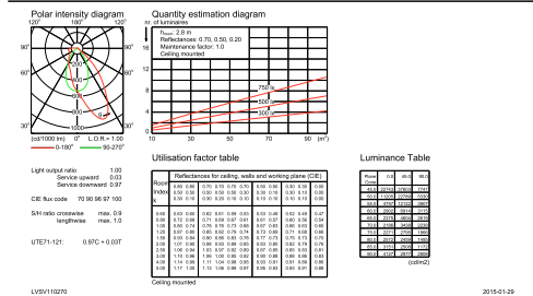
IFGU_4MX900 G3 581 1xLED75S/840 PSD A30-General uniform lighting
